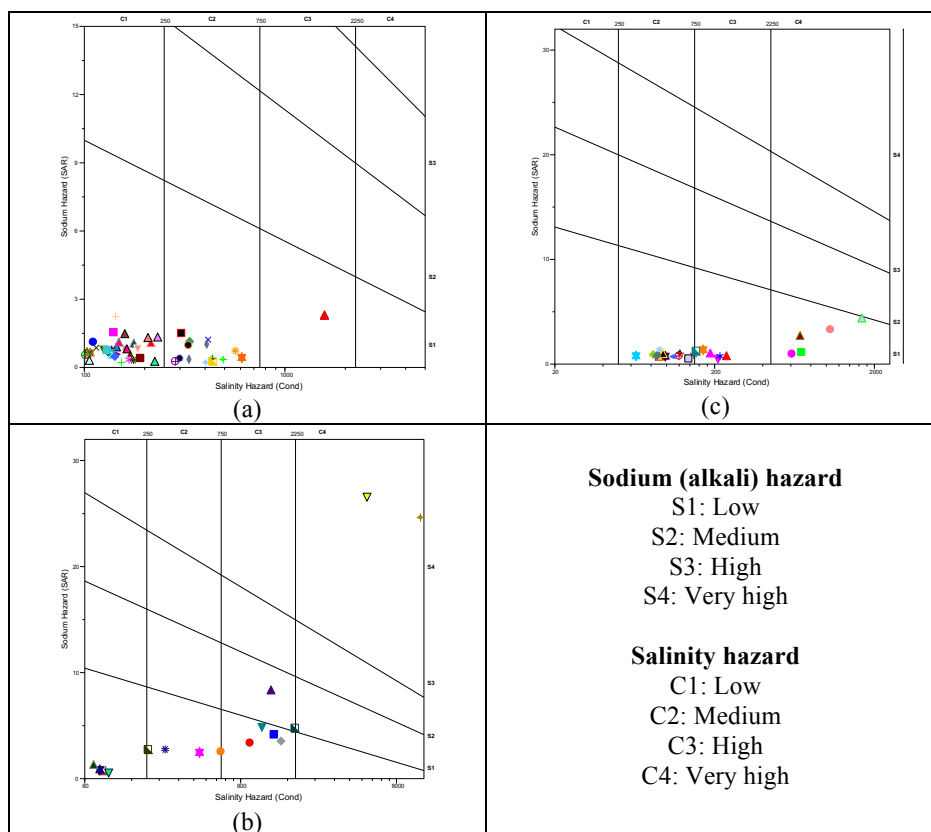
Fig. 3. USSL diagram from (a) shallow, (b) intermediate and (c) deep aquifer for irrigation water quality classification (USSL Diagram 1954)
