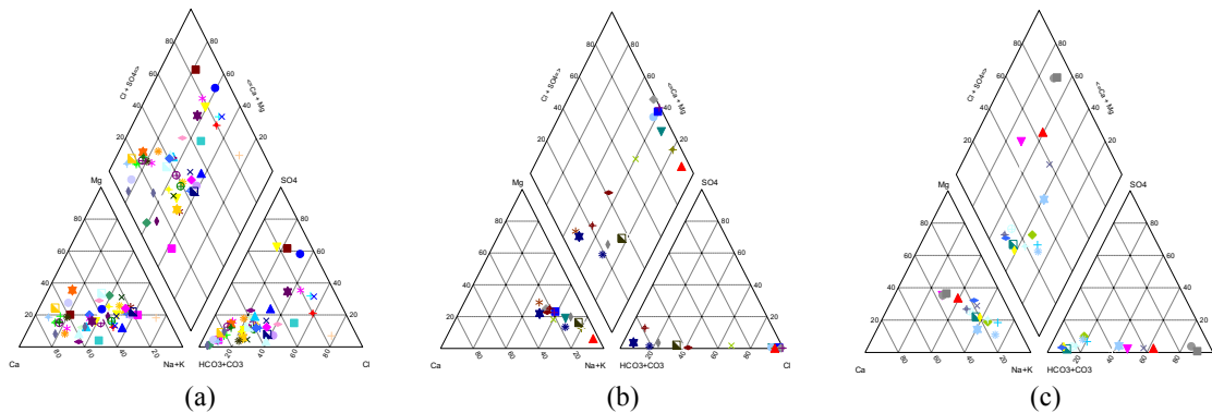
Fig. 2 Piper diagram in (a) shallow groundwater, (b) intermediate groundwater and (c) deep groundwater
